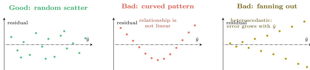
Figure 12.2: Residual plots. Only the left panel is acceptable. A curve means the relationship is non-linear; a fan means the error variance changes with the prediction, so your confidence intervals are wrong even if the coefficients are not.
